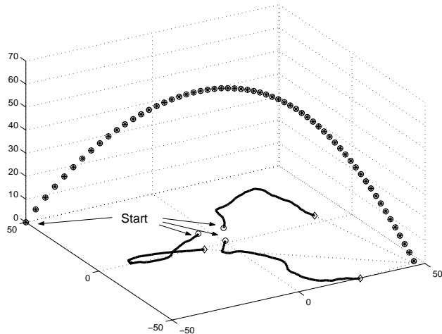
Figure 10: Ground observer trajectories optimally tracking an aerial target.
