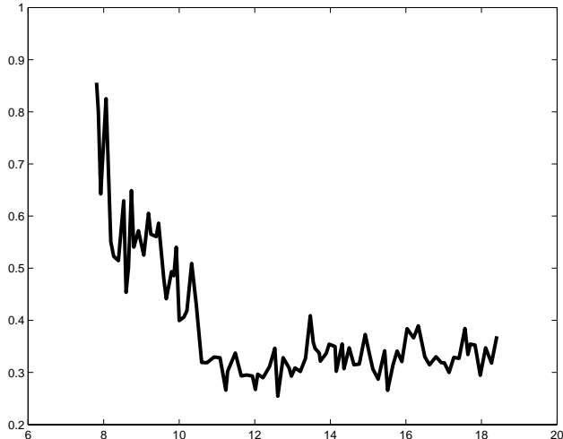
Figure 17: Estimated RMS position error (cm) vs. time for the single target case with obstacles. Results are comparable to the obstacle-free case.
