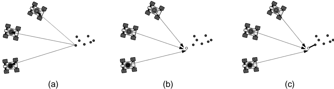
Figure 3: Evaluating Q(\rho) . A sample \omega is taken randomly from P(\omega) and projected into the sensor frames (a), corrupted with noise from our sensor model and reprojected as \hat{\omega} (b), so that Disp(\omega, \hat{\omega}) can be calculated (c). This is repeated for N random samples.
