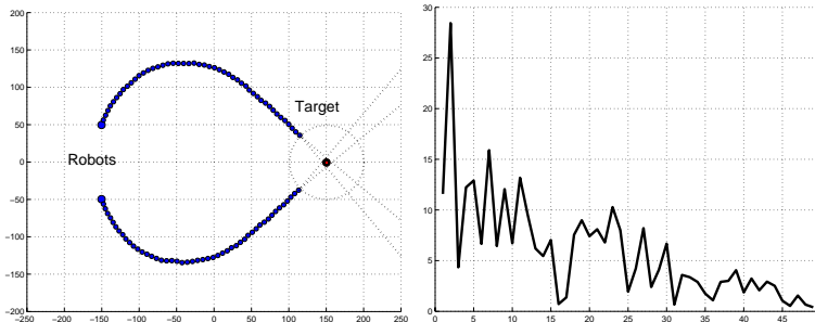
Figure 4: Generated trajectories (left) and disparity measurements for 2 robots tracking a static point target.
