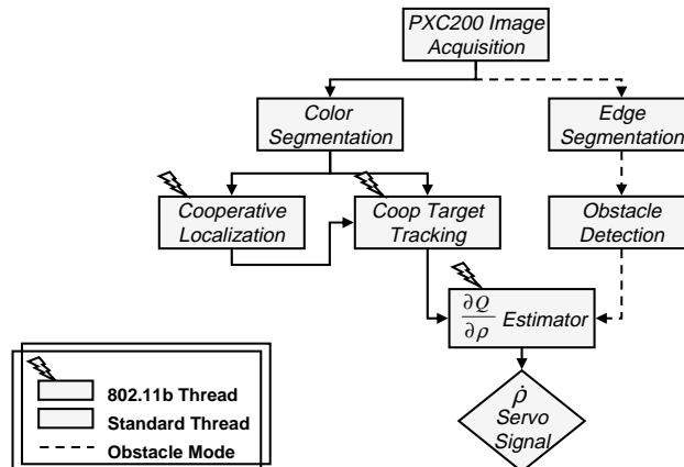
Figure 13: Experimental architecture used by each pursuer. The 802.11b blocks correspond to threads where cooperation - and as a result communication - with other robots is required.
