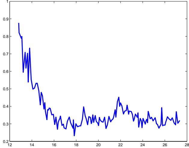
Figure 15: Estimated RMS position error (cm) vs. time for the single target case.
