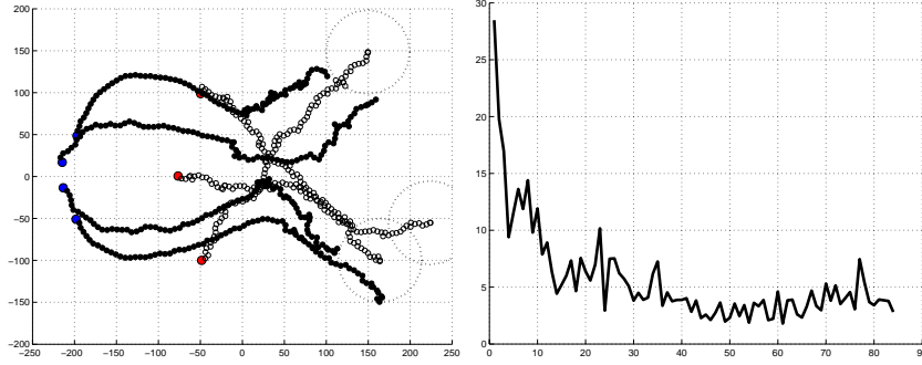
Figure 7: Generated trajectories and summed disparity measurements for 4 robots tracking 3 point targets.
