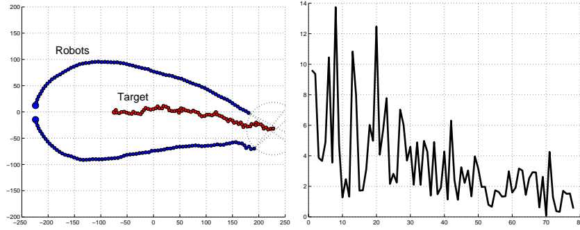
Figure 5: Generated trajectories (left) and disparity measurements for 2 robots tracking an unpredictable moving point target.
