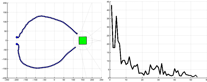
Figure 8: Generated trajectories and summed disparity measurements for 2 robots tracking a static box.
