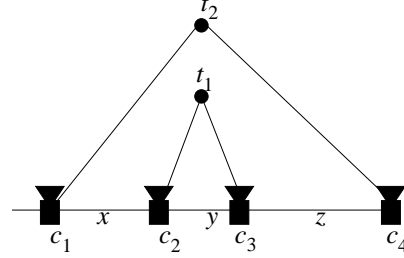
Fig. 4. Figure for lemma 8
