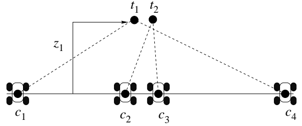
Fig. 1. A greedy assignment assigns c_1 and c_4 to target t_1 and gets stuck with the pair (c_2, c_3) . The optimal assignment in this case is to assign t_1 to (c_1, c_3) and t_2 to (c_2, c_4) .
