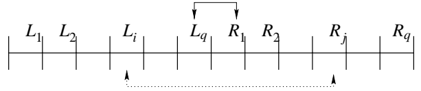
Fig. 3. Partitioning the line segment: A small edge (solid line) and an edge of type (i, j) (dotted line).
